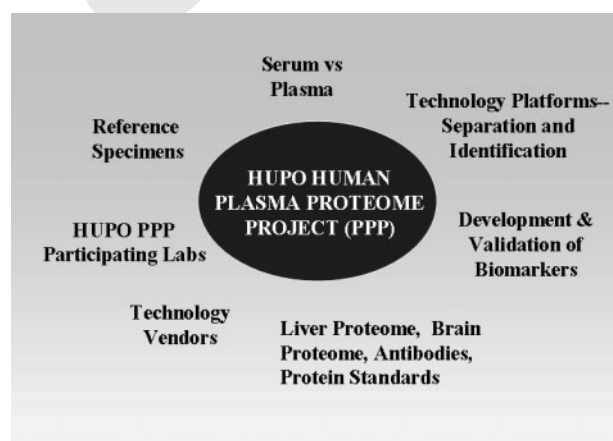
Figure 1. Schema showing relationship of HUPO Plasma Proteome Project (PPP) to other HUPO Initiatives and components of the PPP.
