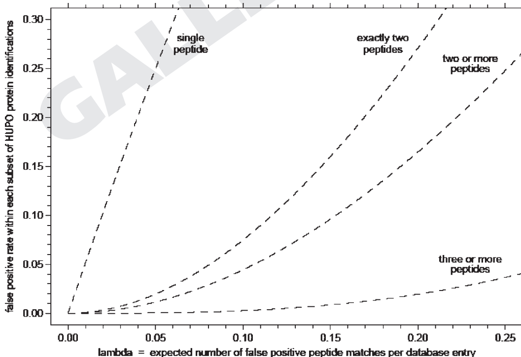
Figure 4. Plot of estimated error rate for subsets of PPP proteins based on one, two, or three or more peptides, Poisson model.
